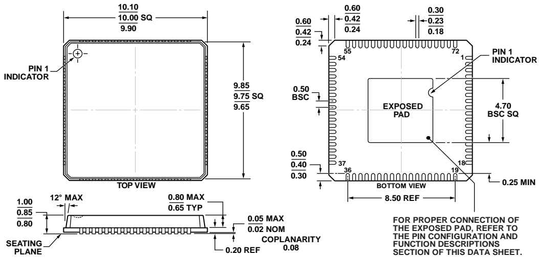
COMPLIANT TO JEDEC STANDARDS MO-220-VNND-4 Figure 66. 72-Lead Lead Frame Chip Scale Package [LFCSP_VQ] 10 mm × 10 mm Body, Very Thin Quad (CP-72-1) Dimensions shown in millimeters
