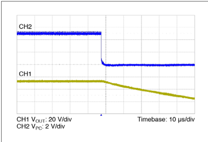
Figure 13 – PC disable waveform, 270 V IN , 100 μF C OUT full load
